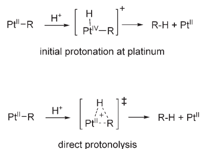
Scheme 8. Oxidative and non-oxidative modes for the protonolysis of the Pt–C bond.
