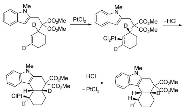
Scheme 5. Outer-sphere nucleophilic attack of indole on a Pt-coordinated olefin (deuterium labeled) in a catalytic intramolecular hydroarylation process.
